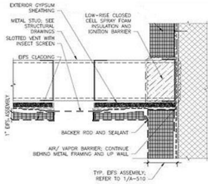
2 EIFS TRANSITION AT LOWER SOFFIT 3" = 1'-0"
