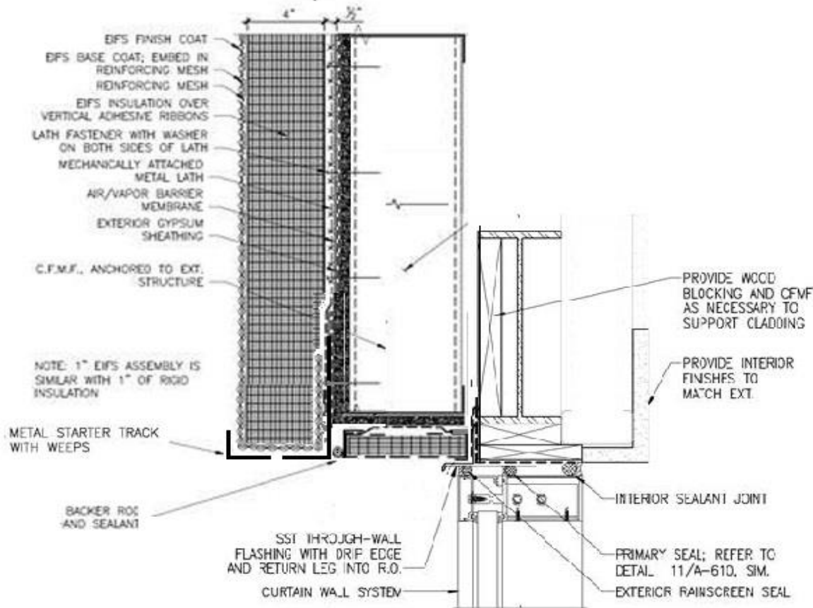
4 CLERESTORY WINDOW HEAD DETAIL
