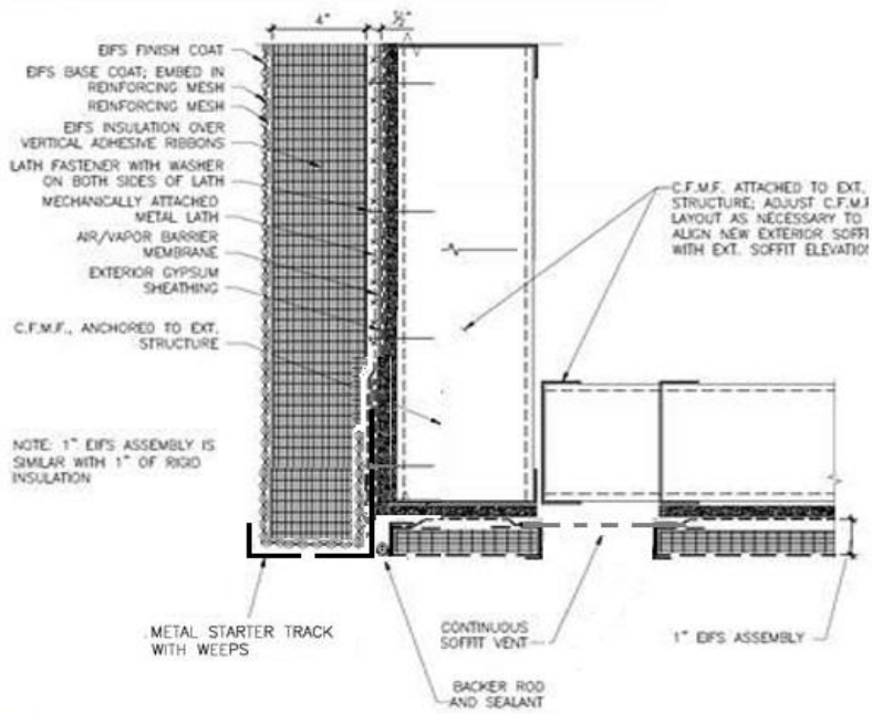
3 LOWER SOFFIT OUTSIDE CORNER 3" = 1'-0"
