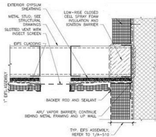
2 EIFS TRANSITION AT LOWER SOFFIT 3" = 1'-0"
